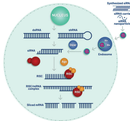
RNA Interference
